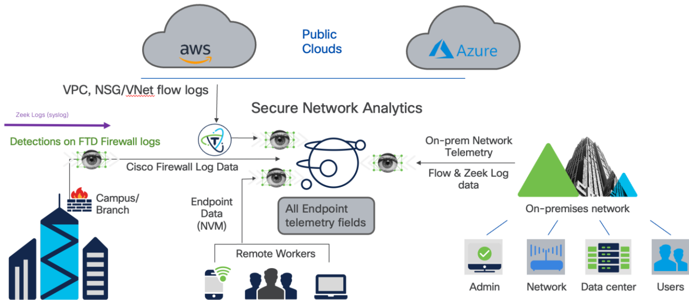
Figure 2. Multi-telemetry ingest
