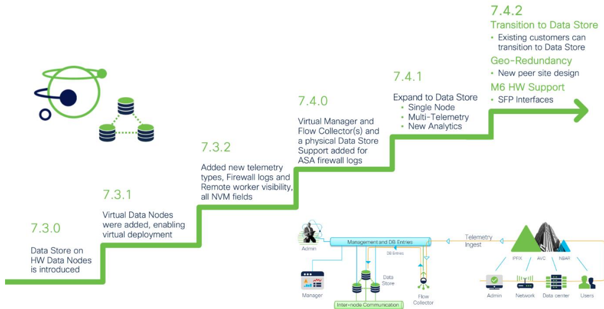
Figure 1. Data Store advancements by version
