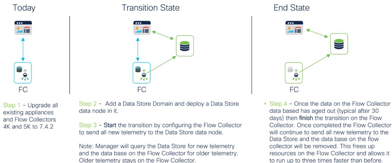
Figure 24. Transitioning from a Flow Collector to a Data Store architecture
