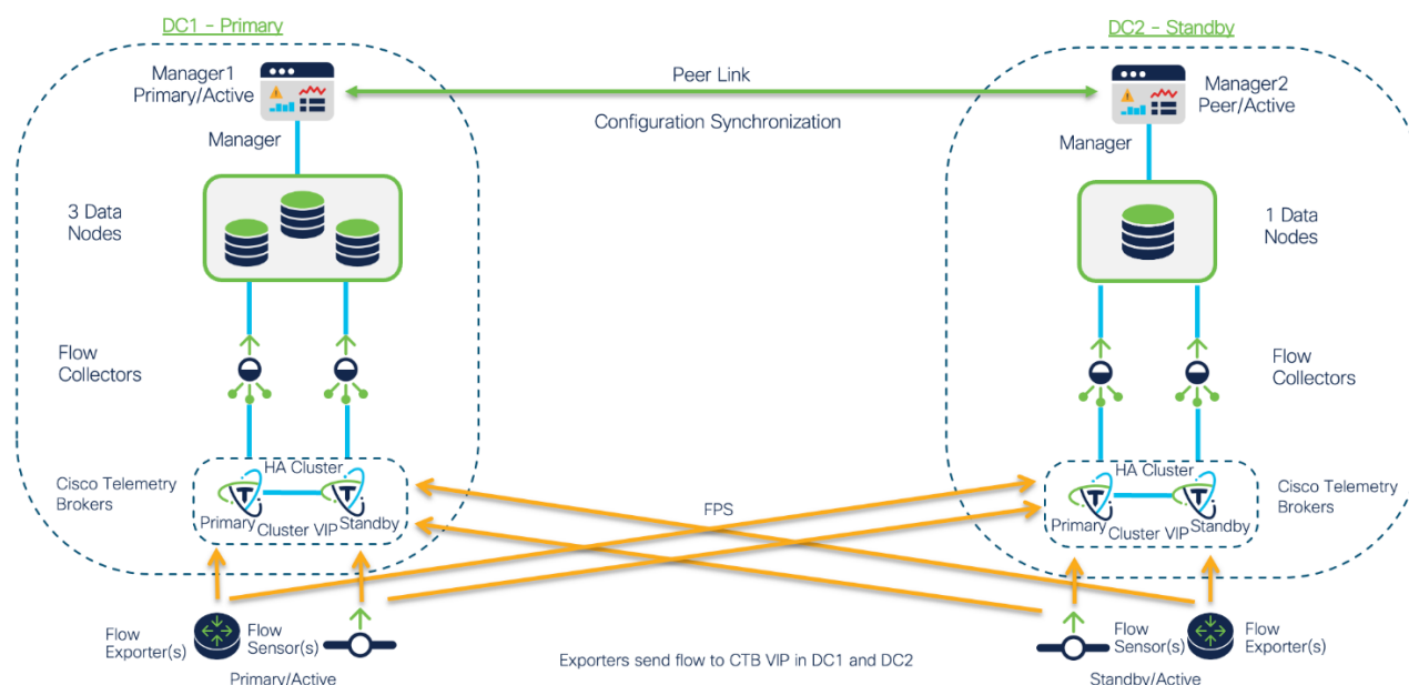
Figure 23. Redundant 3 node and 1 node Data Stores in peer site data centers
