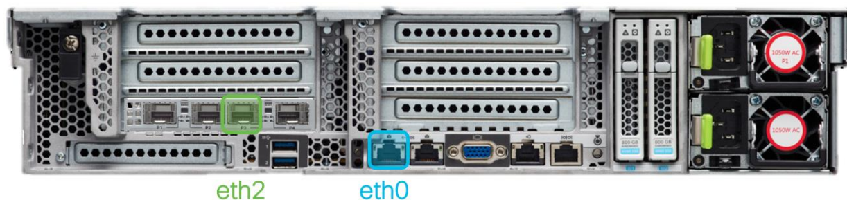
Figure 13. DS6200 mixed mode management configuration option
