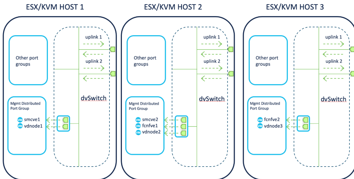
Figure 18. Management communications across a virtual 3 node deployment
