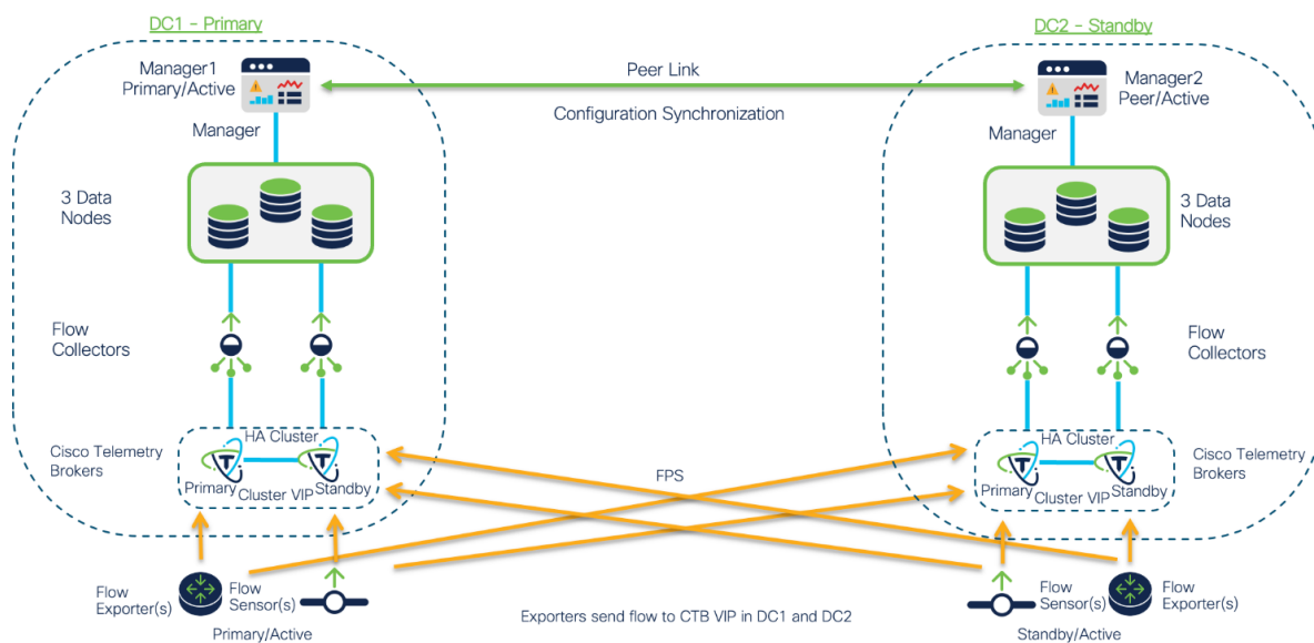
Figure 22. Redundant 3 node Data Stores in peer site data centers
