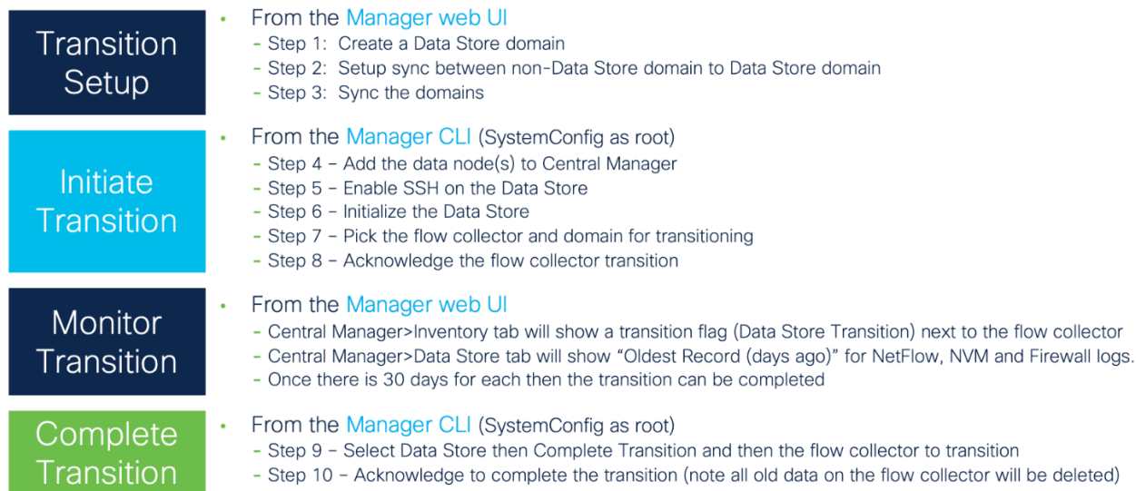
Figure 25. How to transition to the Data Store architecture
