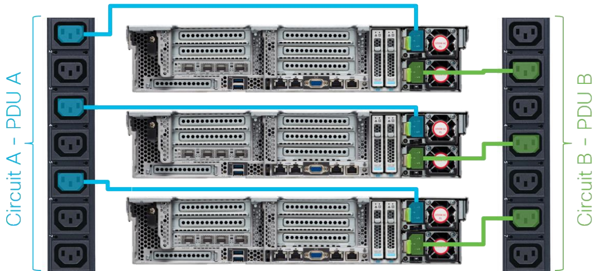
Figure 15. DS6200 power redundancy
