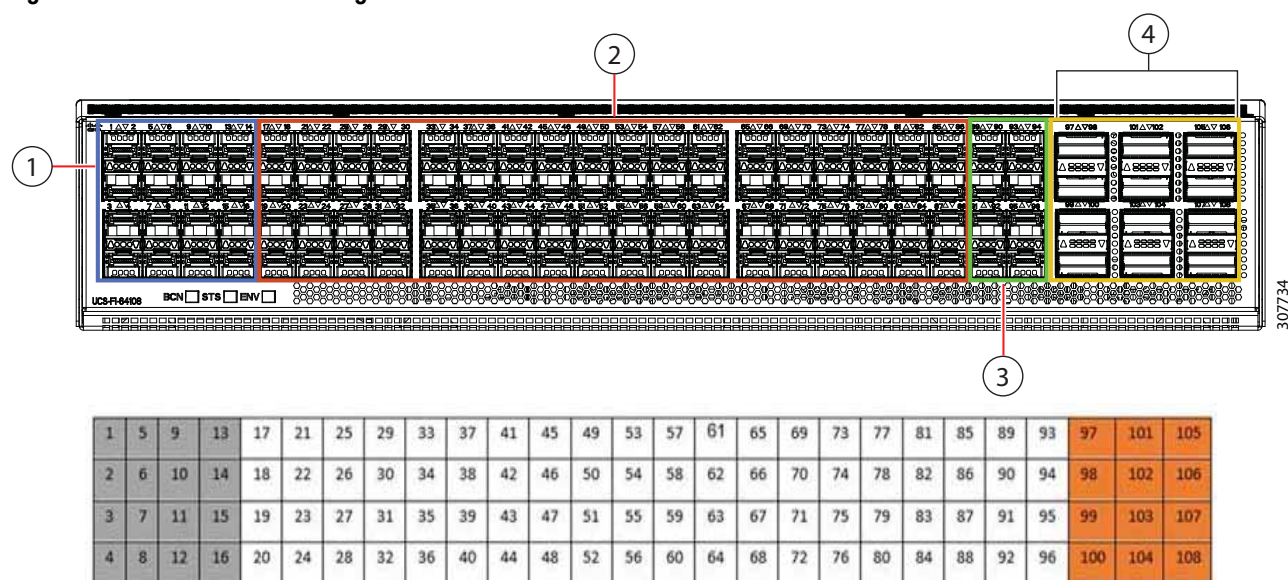
Figure 16 Port Numbering of the Cisco UCS 64108
