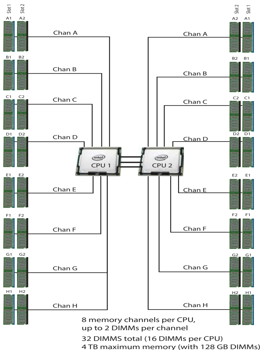
Figure 6 C220 M6 SFF Memory Organization
