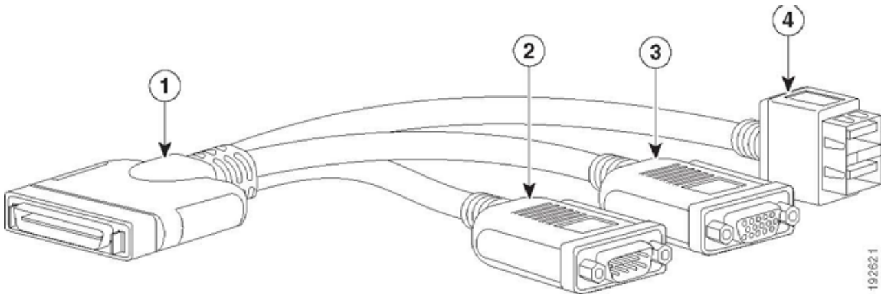
Figure 14 KVM Cable
